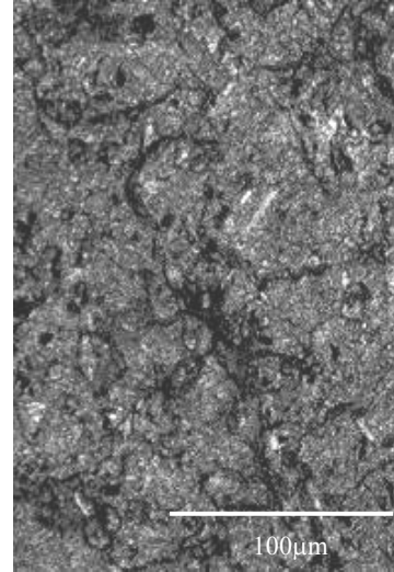
(b) Fracture surface of Mode I fatigue crack growth.
