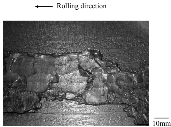
Fig.1 Small spalling of the hot rolling mill roll.
