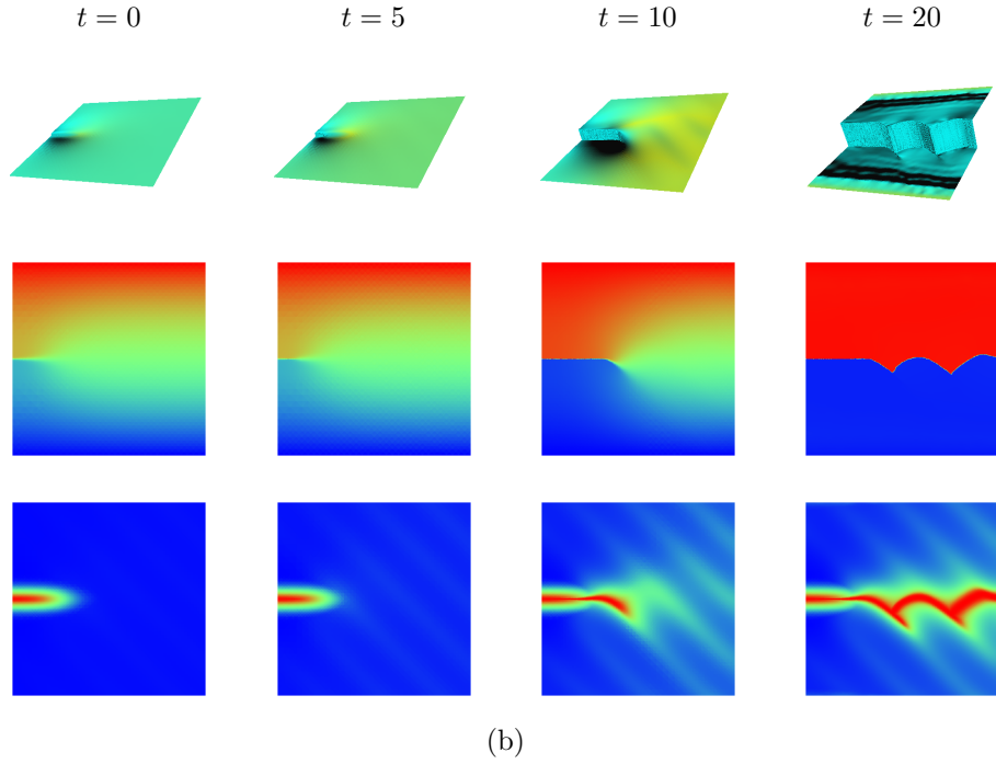
Figure 4: Birdviews of u(\text{top}) , u (middle) and z (bottom) in the temporal evolution of the cracks when (a) \gamma(x) = 0.5(1 + 0.2 \cos 10x \cdot \cos 10y) and (b) \gamma(x) = 0.5(1 + 0.2(\cos 10x + \cos 10y)) .
