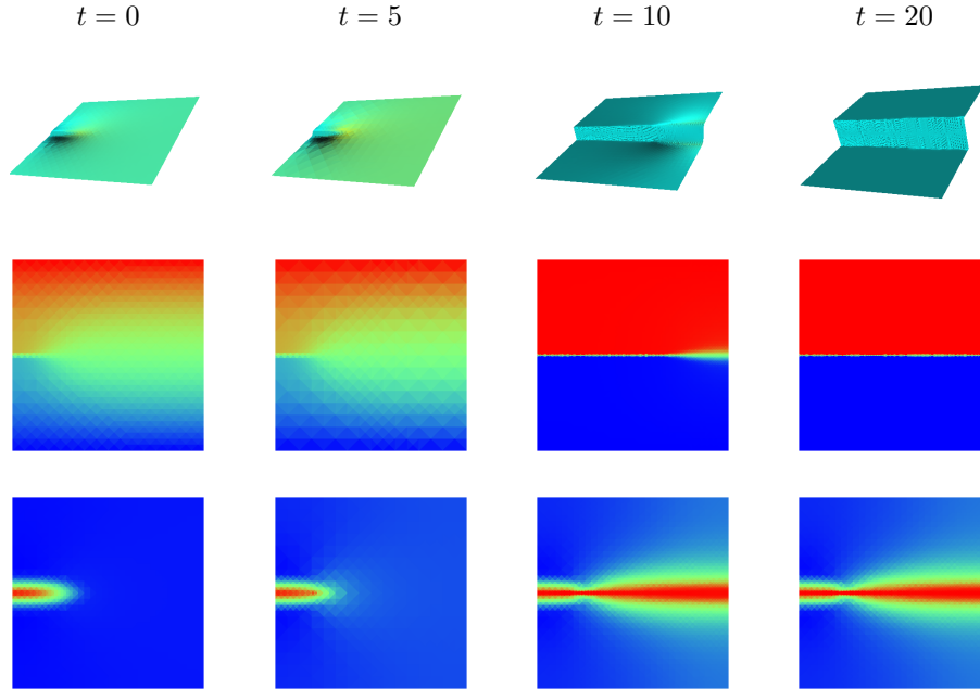
Figure 1: Birdviews of u (top), u (middle) and z (bottom).
