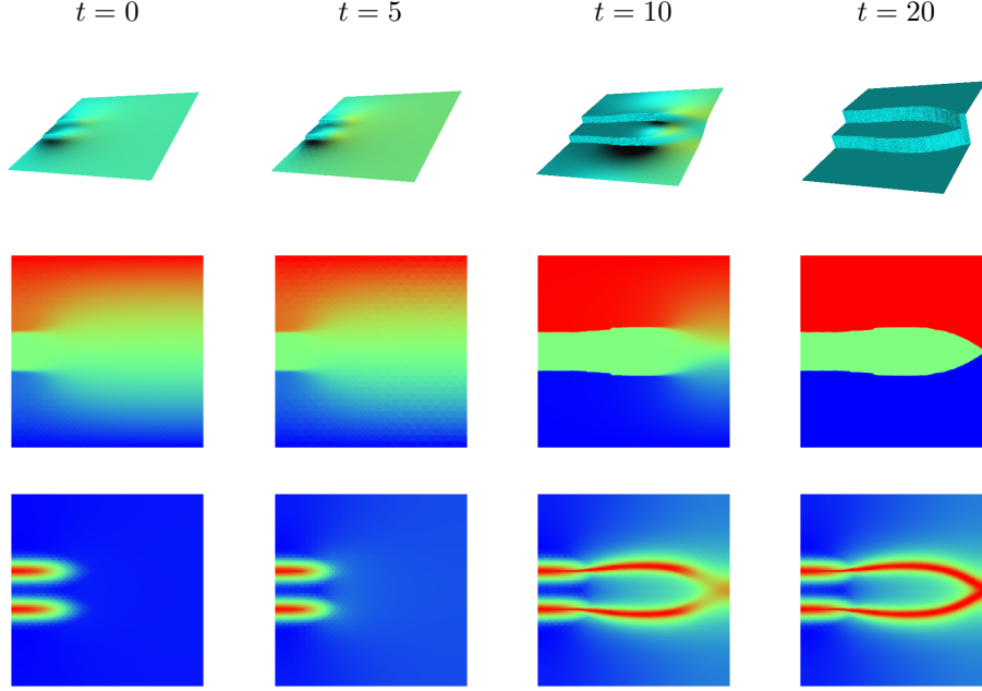
Figure 2: Birdviews of u (top), u (middle) and z (bottom) in the temporal evolution of the cracks when initial length of cracks is 0.5.
