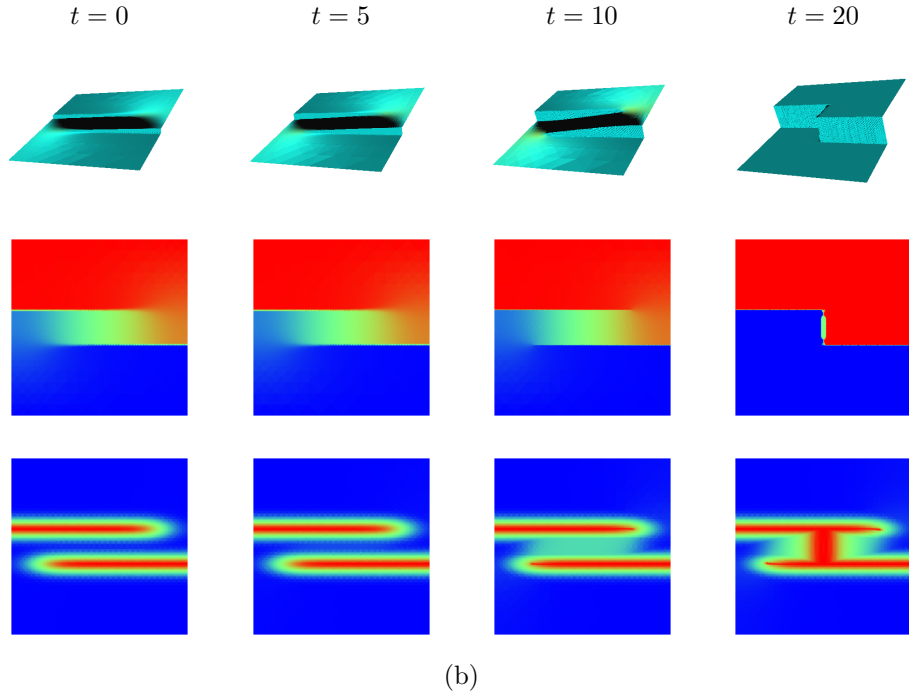
Figure 3: Birdviews of u (top), u (middle) and z (bottom) in the temporal evolution of the cracks with initial cracks of length (a) 1.8 and (b) 1.7 .
