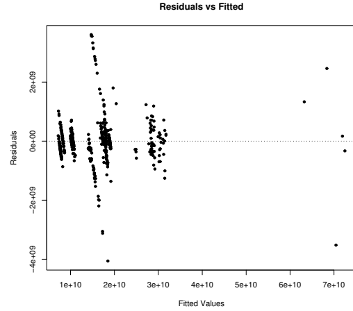
Fig. 4. Residual plot for model in Tab.3
