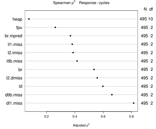
Fig. 2. Strengths of marginal relationships
