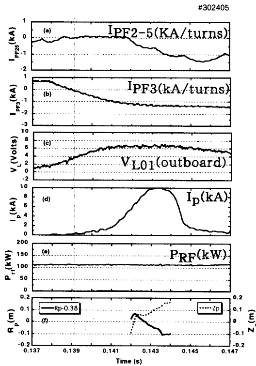
Fig. 2 Plasma current start-up in TST-2 at B_t=0.28 T with the first coil arrangement, with (a) PF2 and PF5 coil current (connected in series), (b) PF3 coil current, (c) loop voltage measured on the outboard side of the torus, (d) plasma current, (e) injected and reflected RF powers, and (f) horizontal and vertical positions of the plasma current centroid. The current start-up time is indicated by the vertical line.
