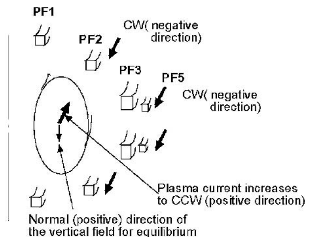
Fig. 1 Schematic of the TST-2 plasma cross section and poloidal field coils.
