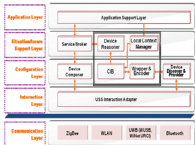
Figure 4. The Architecture of the Middleware for Device Sharing
