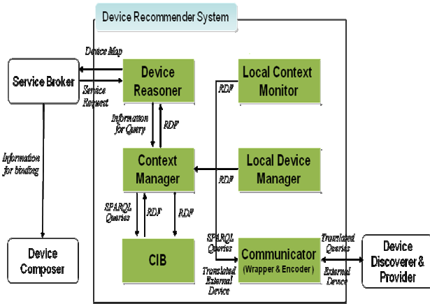
Figure 5. The Architecture of Device Recommender System
