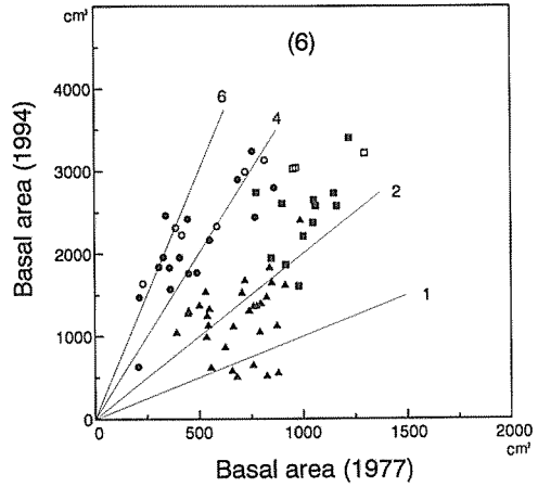
Fig. 3-4 Relation between basal area of six trees-clump in 1977 and that in 1994. 1, 2, 4, 6 : Ratio of basal area in 1994 to basal area in 1977. Symbols : Refer to Fig. 3-2.
