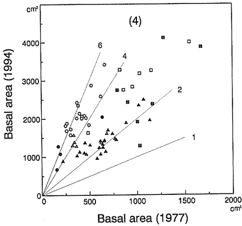
Fig. 3-3 Relation between basal area of four trees-clump in 1977 and that in 1994. 1, 2, 4, 6 : Ratio of basal area in 1994 to basal area in 1977. Symbols : Refer to Fig. 3-2.
