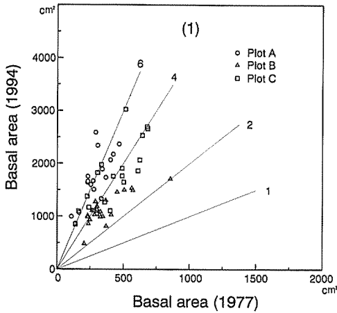
Fig. 3-1 Relation between basal area of single tree-clump in 1977 and that in 1994.
