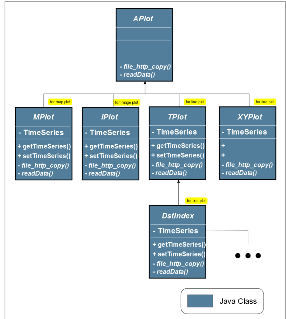
Deployment Diagram 1 (Judass)
