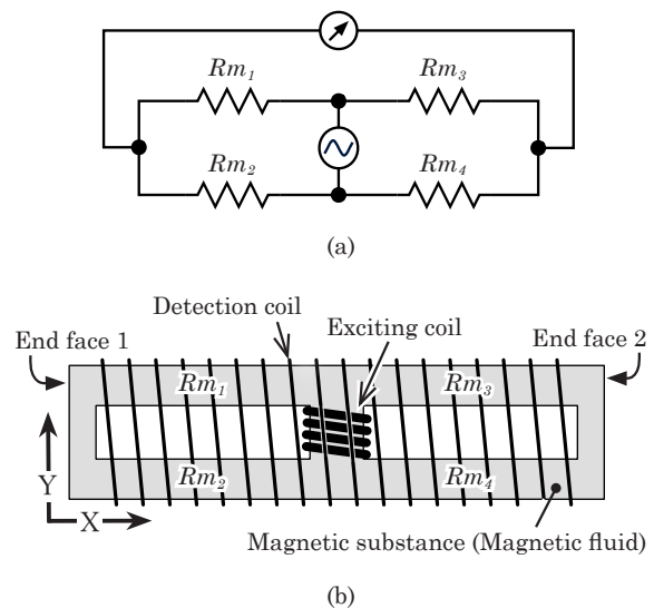
Fig. 2 Wheatstone bridge circuit representation of a magnetic bridge (a) and a basic structure of a magnetic bridge (b), in which Rm_1 \sim Rm_4 are magnetic reluctance on the each branch.
